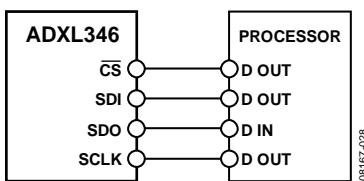
Figure 35. 4-Wire SPI Connection Diagram
